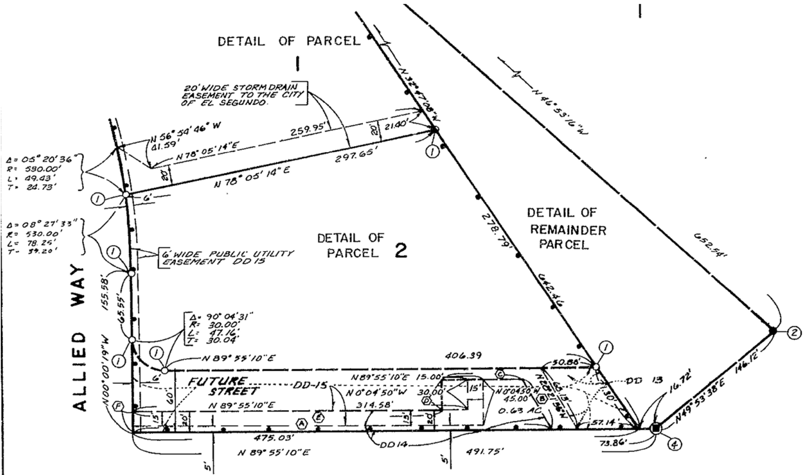
DETAIL "A" SCALE 1" = 50'
