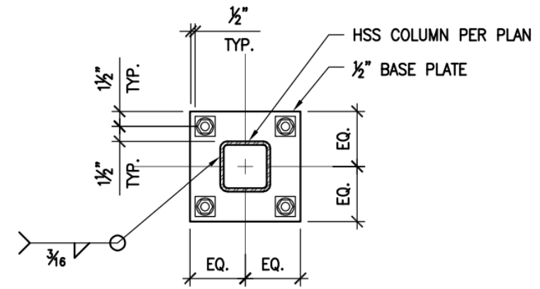
E: FOUR BOLT PATTERN
